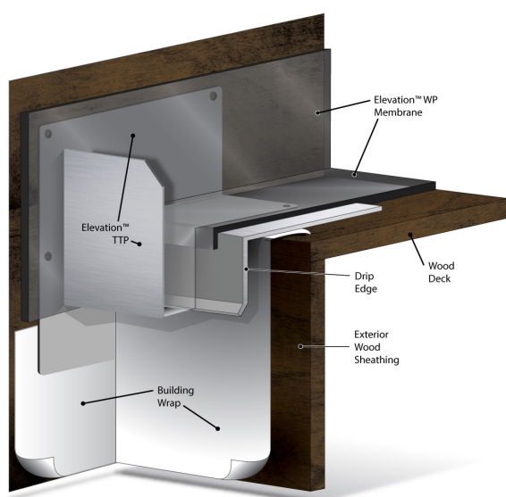
DETAIL
